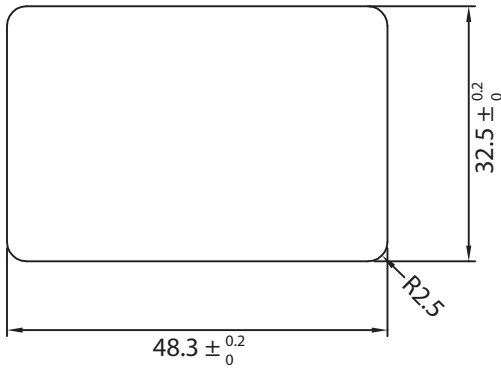
PANEL CUTOUT
